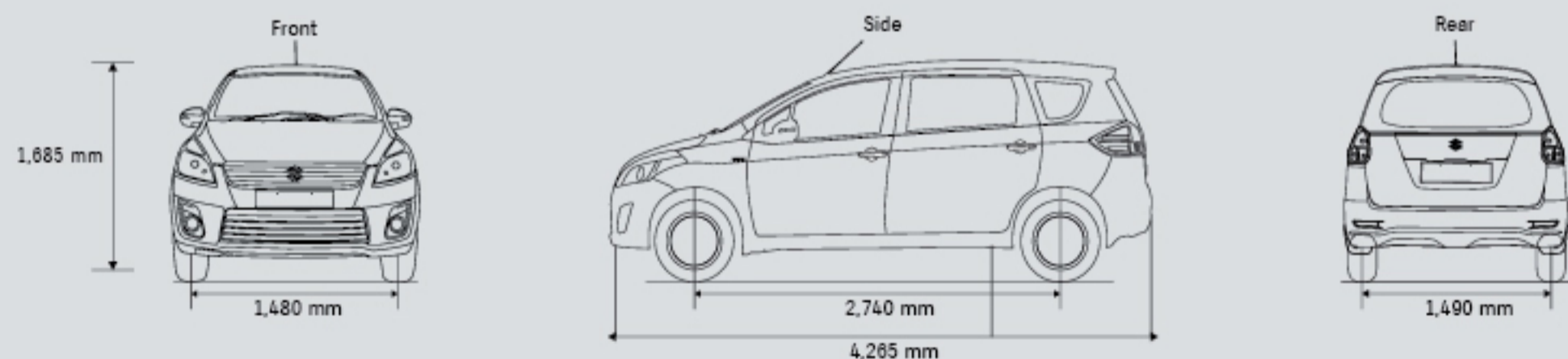
Car Line Drawings
