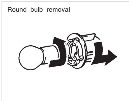
Front clearance/turn signal lights
