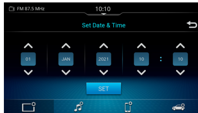
Figure 13: Set Date &amp; Time Dialog Box - 24 Hour Format
