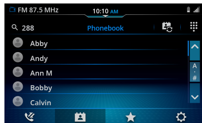
Figure 41: Phonebook Screen
