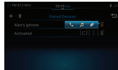
Figure 40: Paired Devices
