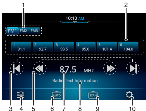
Figure 33: Radio/Tuner Screen
