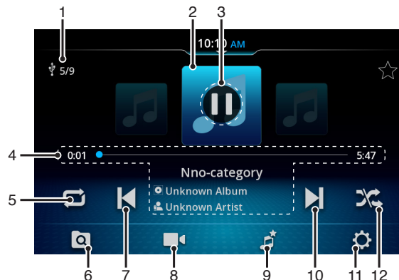
Figure 53: Media Screen
