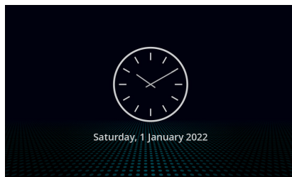
Figure 7: Wallpaper Mode
