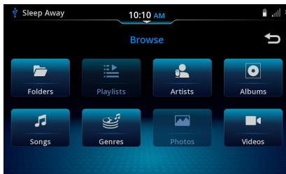
Figure 54: Browse Screen
