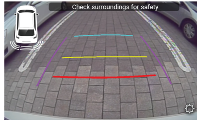
Figure 77: RVC Screen
