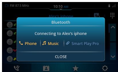
Figure 37: Pairing Successful
