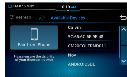
Figure 34: Available Devices
