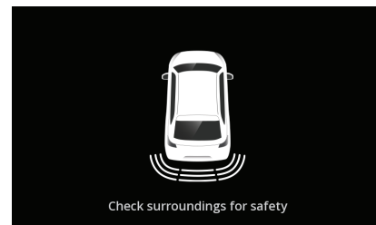
Figure 76: RPAS Screen
