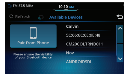
Figure 34: Available Devices
