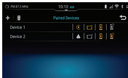
Figure 40: Paired Devices
