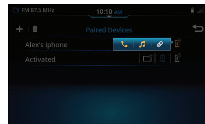
Figure 41: Paired Devices
