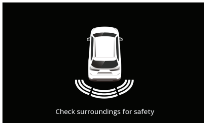
Figure 80: RPAS Screen
