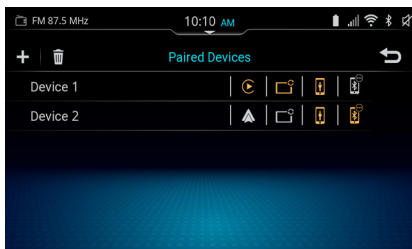
Figure 59: Paired Devices
