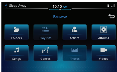
Figure 55: Browse Screen
